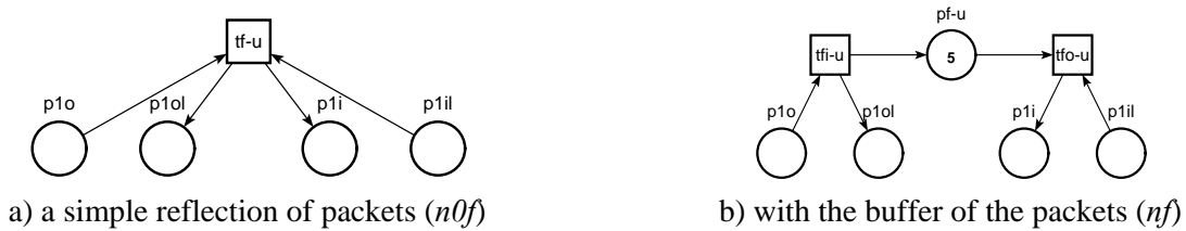
Figure 2 – Petri net models of a terminal device
